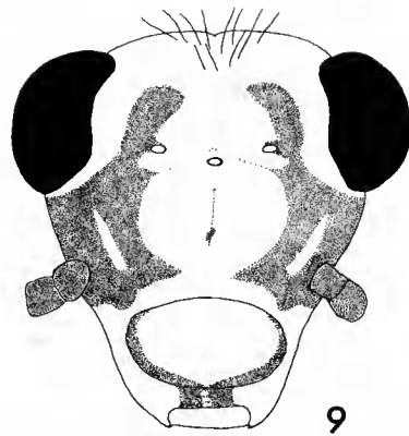
FIGS 3-9. — Echmepteryx gumpi , ♂ holotype : 3, fore wing; 4, hypandrium; 5, phallosome. ♀ allotype : 6, head; 7, gonapophyses. Lepidopsocus pretiosus ♀ : 8, head. Lepidopsocus sp., nymph : 9, head. (Figs 4, 5 and 7 to common scale, heads not to scale.)
